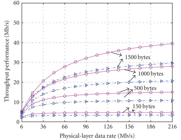
(a) Throughput at different physical-layer data rates
