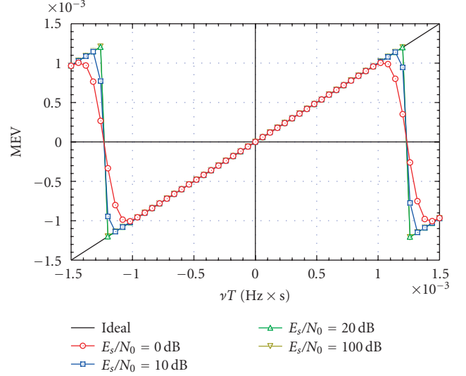
FIGURE 2: MEV of FEPE estimator for different values of E_s/N_0 —simulation only. Preamble + postamble DA ML phase estimation, N = 44 , M = 385 .
