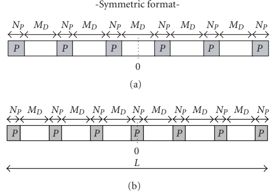
FIGURE 12: Generic symmetric burst format.
