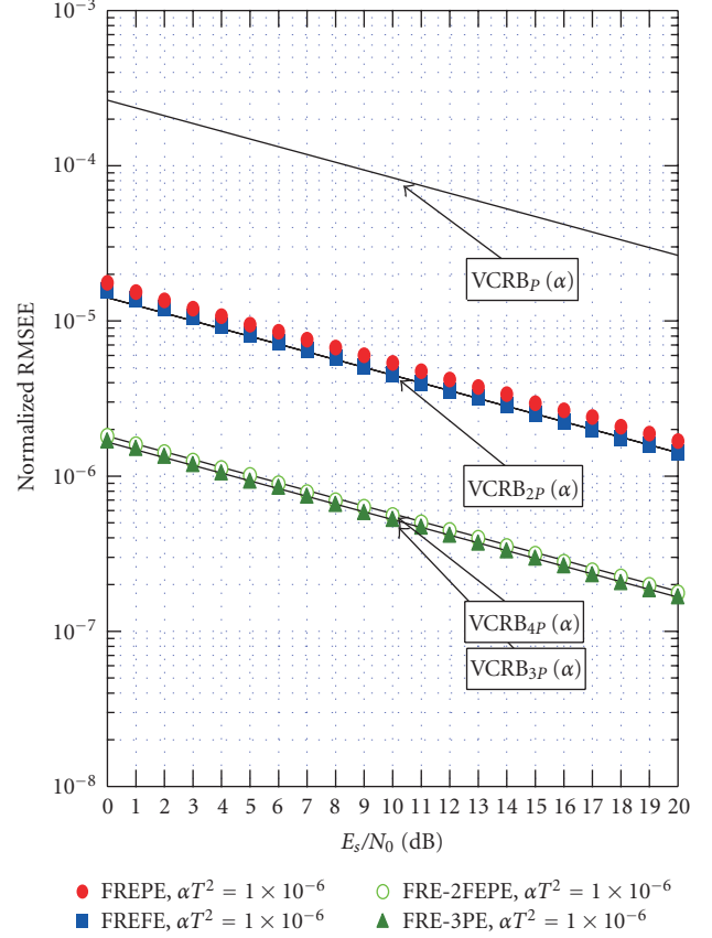
FIGURE 9: RMSEE of FREPE, FREFE, FRE-3PE, and FRE-2FREPE estimators for different values of E_s/N_0 and relevant bounds,—solid lines: theory—marks: simulation. Doppler-rate algorithms: FREFE versus FREPE versus FRE-3PE versus FRE-2FEPE, N = 44(45) , M = 385(384) , \nu T = 1.0 \times 10^{-3} .
