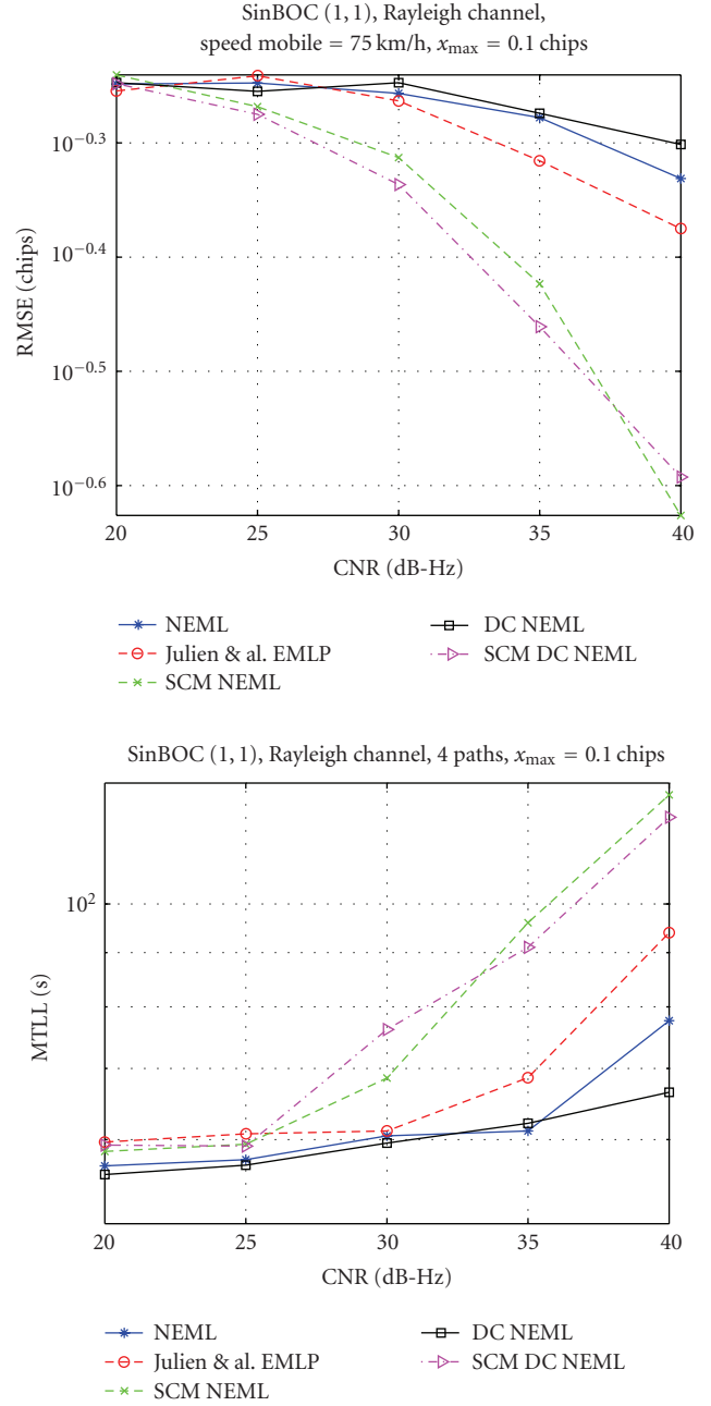
FIGURE 19: Comparison of feedback delays estimation algorithms employing the NEML discriminator and of the Julien&al. method, as a function of CNR; SinBOC(1, 1) modulation, Rayleigh channel with an average pathpower delay profile of -1, -2, 0, and -3 dB, v = 75 km/h, closely spaced paths with x_{\max} = 0.1 chips.
