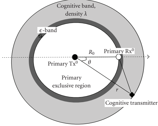
FIGURE 5: Worst-case interference to a primary receiver: the receiver is on the boundary of the primary exclusive region of radius R_0 . We seek to find R_0 to satisfy the outage constraint on the primary user.
