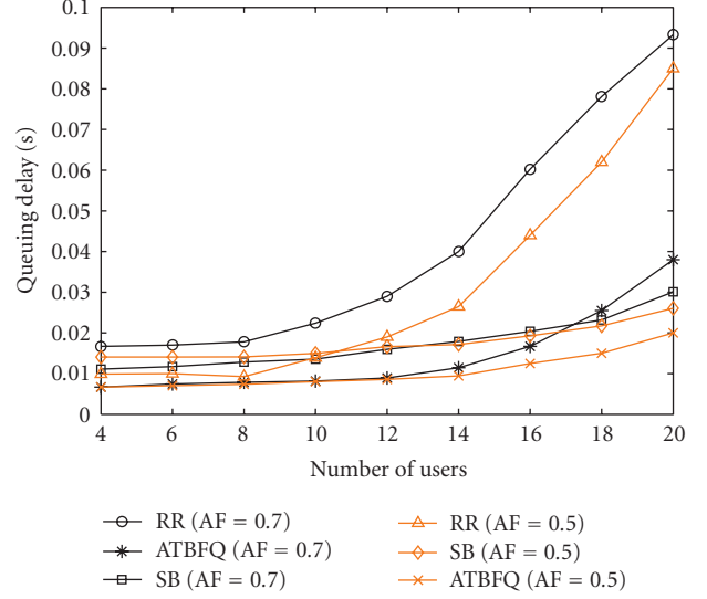
FIGURE 8: Average UT queuing delay versus number of UTs.
