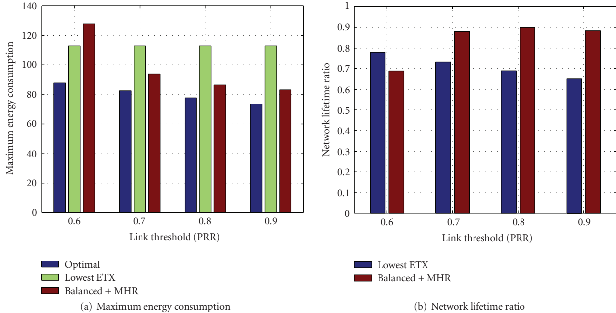
FIGURE 15: Comparison of the lowest ETX scheme and the balanced scheme in terms of (a) the maximum energy consumption and (b) the network lifetime normalized to the optimal network lifetime.
