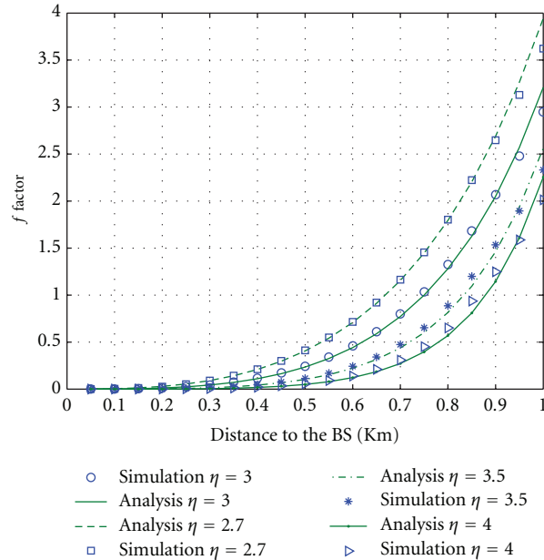
FIGURE 4: OCIF versus distance to the BS; comparison of the fluid model with simulations on a hexagonal network with \eta = 2.7, 3, 3.5 , and 4.
