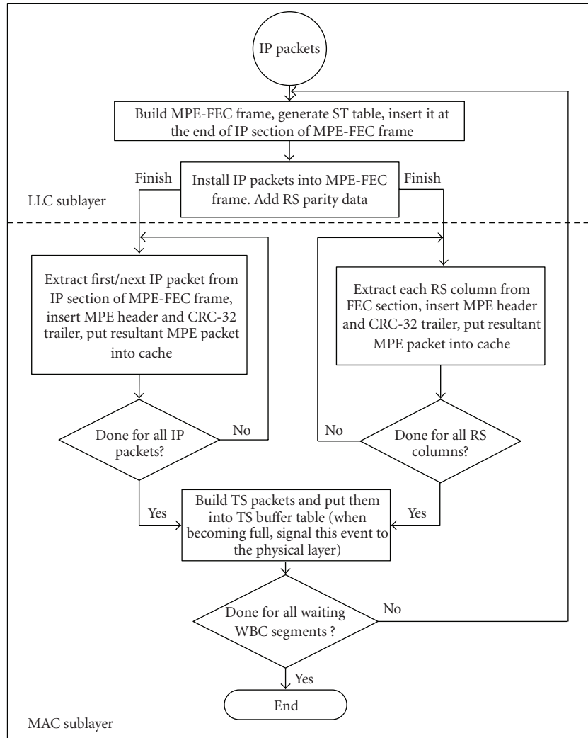
FIGURE 10: The “WBC over DVB-H” link layer encoder’s functional model.
