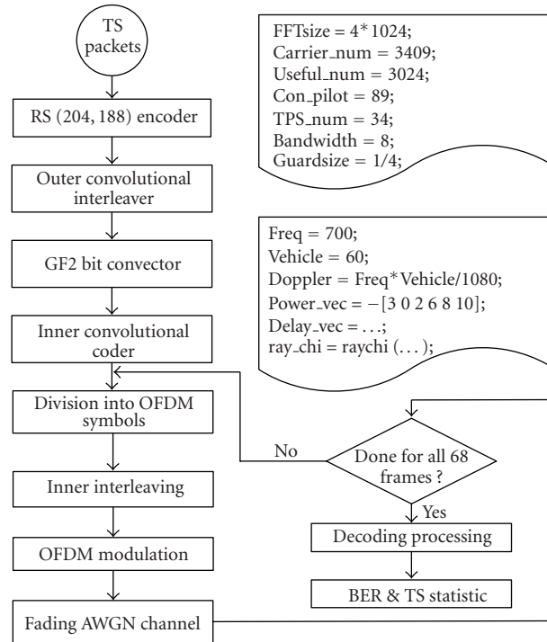
FIGURE 11: The “WBC over DVB-H” physical layer testbed.
