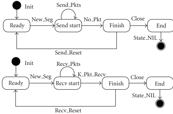
FIGURE 9: The ADP send/receive finite state machine.
