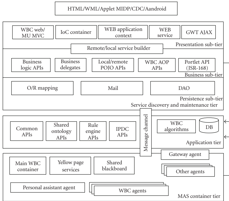
FIGURE 8: The WBC application enabler sublayer’s architecture.
