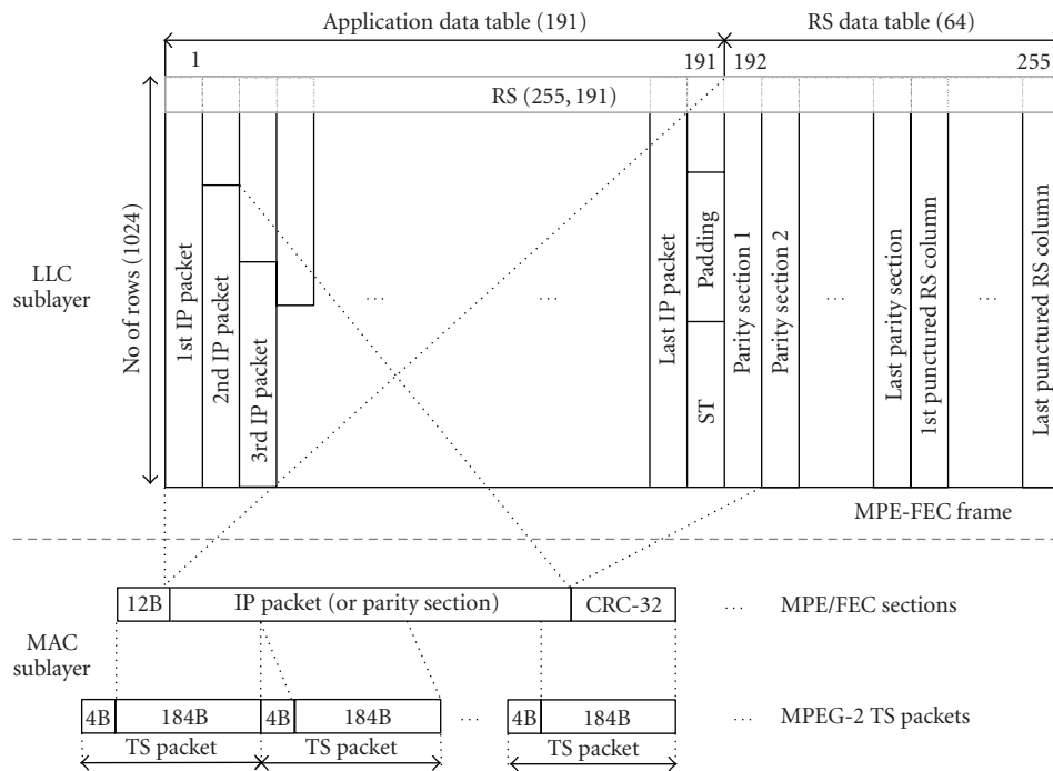
FIGURE 7: The ‘‘WBC over DVB-H’’ link layer PDU encapsulation.
