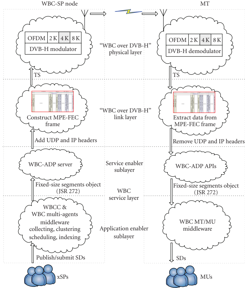
FIGURE 1: The “WBC over DVB-H” layered architecture.
