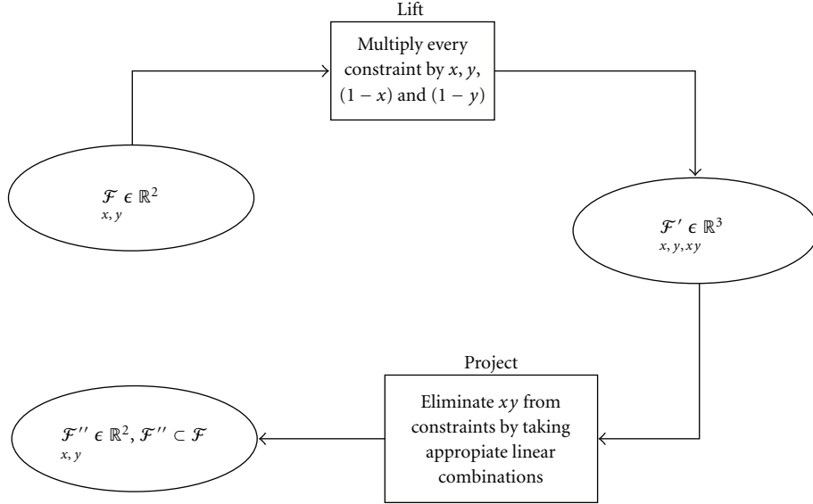
FIGURE 1: Illustration of lift-and-project method for a problem with 2 optimization variables.
