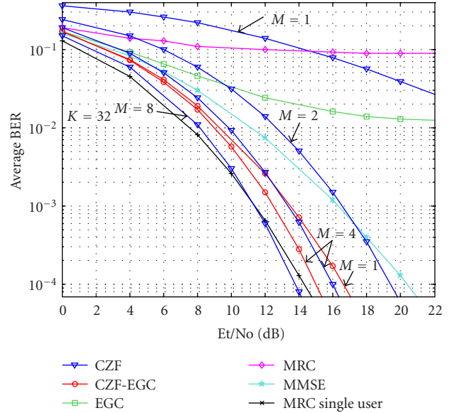
FIGURE 4: Performance comparison between the CZF, CZF-EGC and conventional receivers as function of E_t/N_o , for beamforming case.
