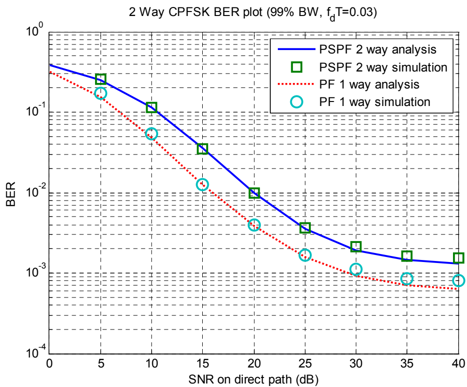
Figure 3 BER of PSPF 2-way 3-phase cooperative transmission in a time-selective Rayleigh fading channel; f_d T = 0.03 ; B_{12} = 1.1818/T and B_3 = 1.832/T .
