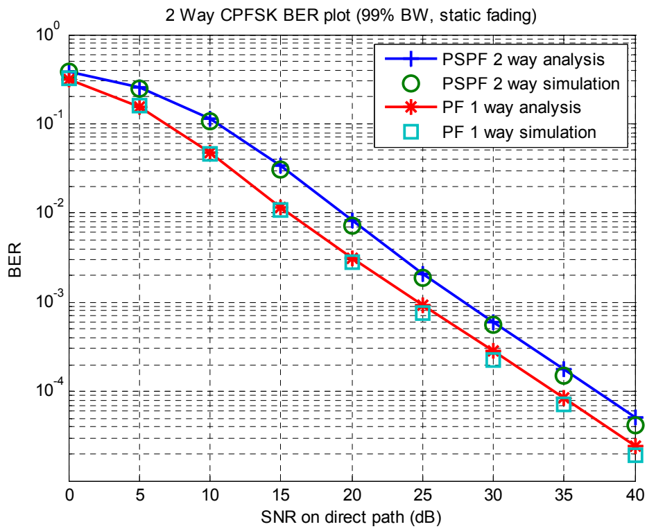
Figure 2 BER of PSPF 2-way 3-phase cooperative transmission in a static Rayleigh fading channel; B_{12} = 1.1818/T and B_3 = 1.832/T .
