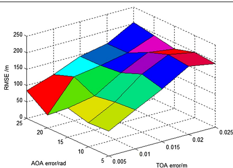
Figure 8 RMSE of different AOA and TOA measurement errors.
