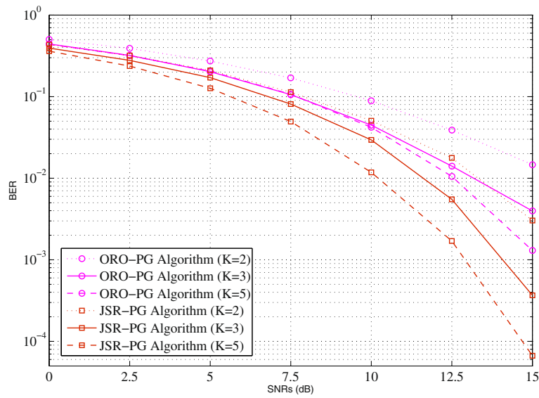
Figure 5 Example 3. BER versus \text{SNR}_s for different K , \text{SNR}_r = 20 dB.
