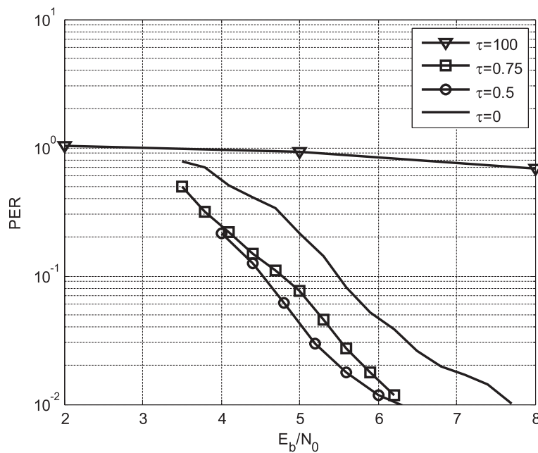
Fig. 11 PER with different decision threshold in AWGN in hopping asynchronous systems with asynchronous symbols. One packet contains 1024 information bits, and one hop has 64 symbols and 16 pilots. Power of each interfering user is 6 dB stronger than that of the desired user
