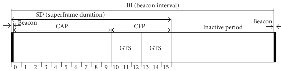
FIGURE 2: Frame structure of the beacon signal in a Zigbee network.
