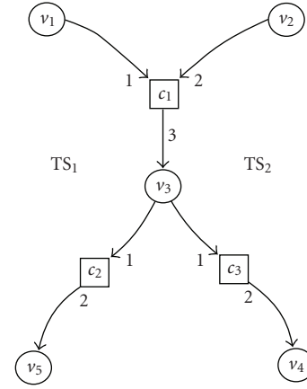
FIGURE 7: Example of common nodes between two trapping sets.
