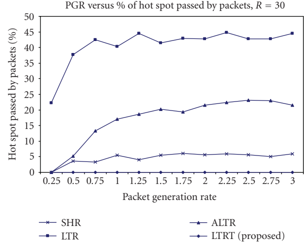
FIGURE 17: Packet generation rate versus number of hot spots passed by packets with radio transmission range 30.
