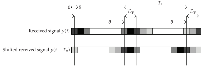
FIGURE 2: Windows used for timing offset estimation.
