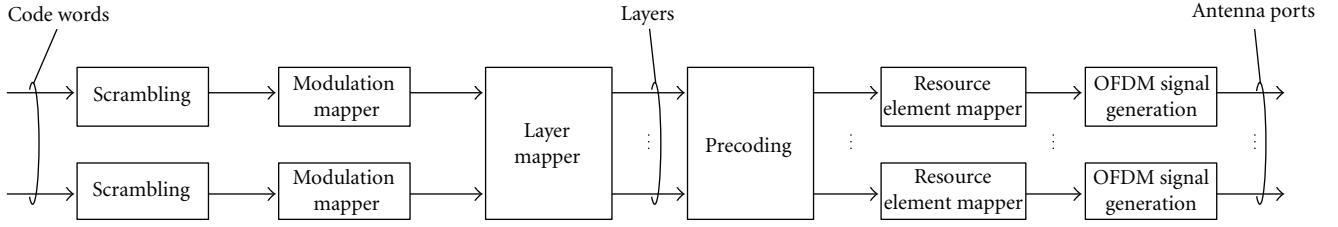
FIGURE 2: Overview of physical channel processing [4].
