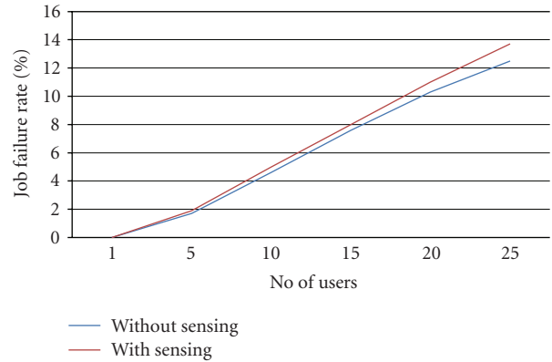
FIGURE 12: Impact of sensing period to MPEG-4 video transmission.
