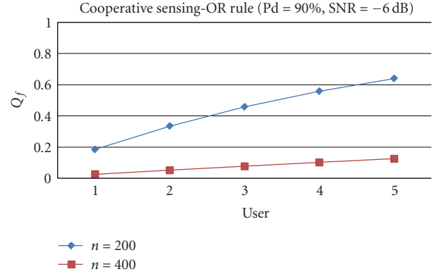
FIGURE 8: Performance of probability of false alarm using OR-rule cooperative sensing under various SNR conditions.
