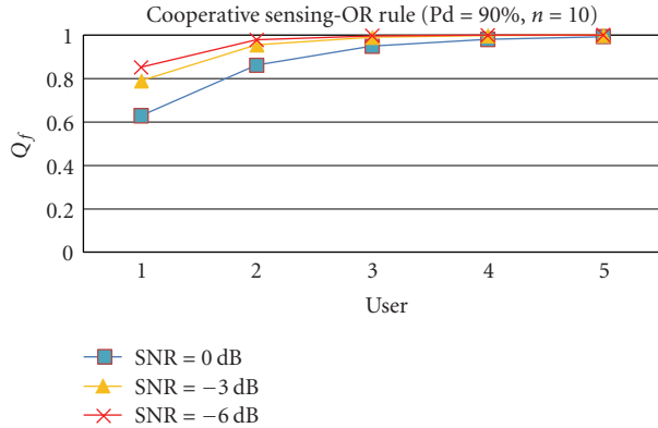
FIGURE 7: Performance of probability of false alarm using OR-rule cooperative sensing under various SNR conditions.
