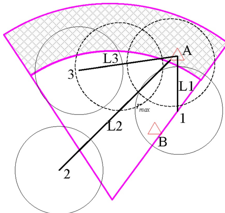
Figure 3 Schematic diagram of border target node coverage.
